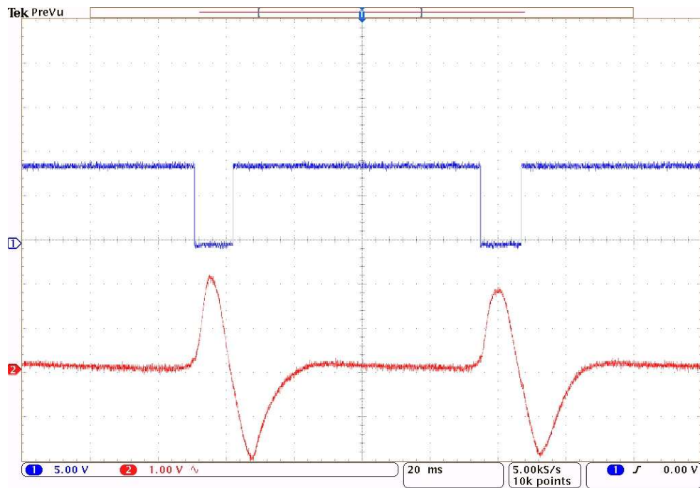
SL EZ Sensor operated by analyser SL MA-110 Trigger signal output (blue, 5V/div.) and analog voltage output (red, 1V/div.).
